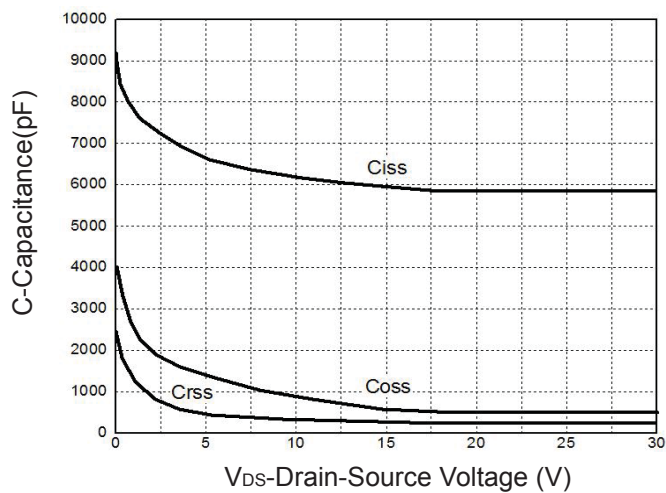
Figure 11: Capacitance Characteristics
