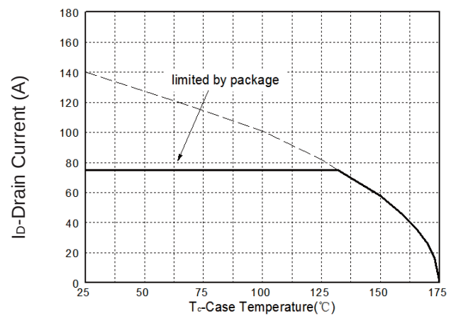
Drain Current
