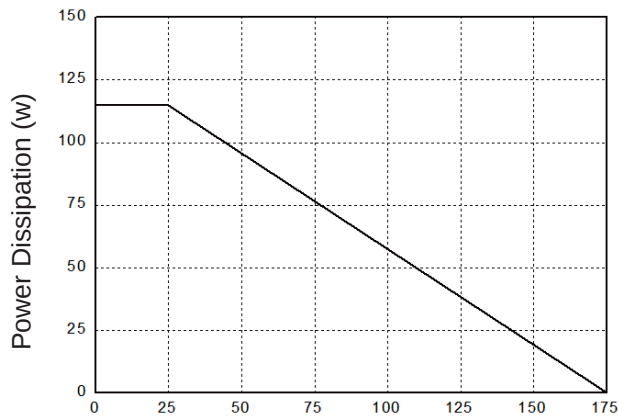
Power Dissipation
