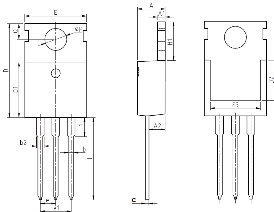
COMMON DIMENSIONS
