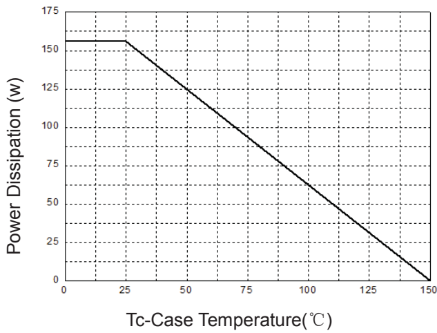
Figure 1: Power Dissipation
