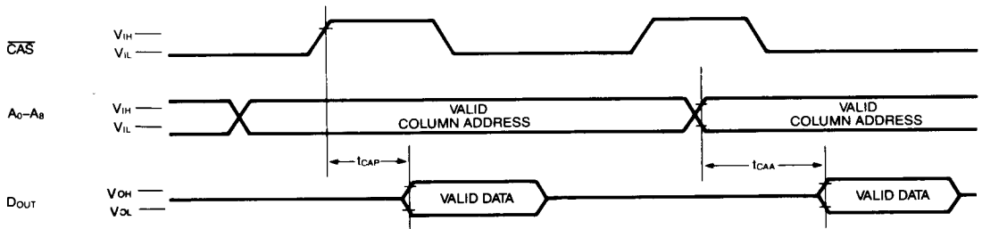
FIGURE 1. FAST PAGE MODE ACCESS TIME DETERMINATION
