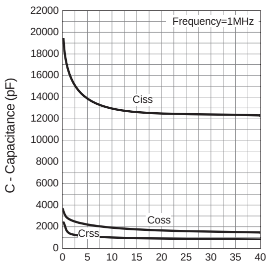
Capacitance
