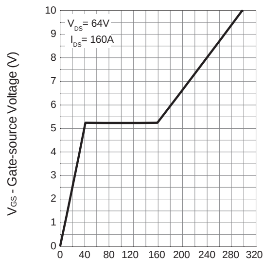
Gate Charge
