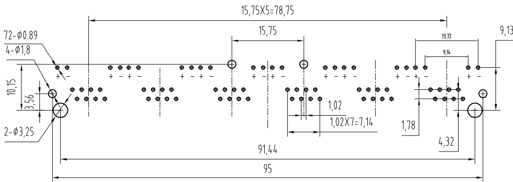
PC Board Layout Component Side Shown
