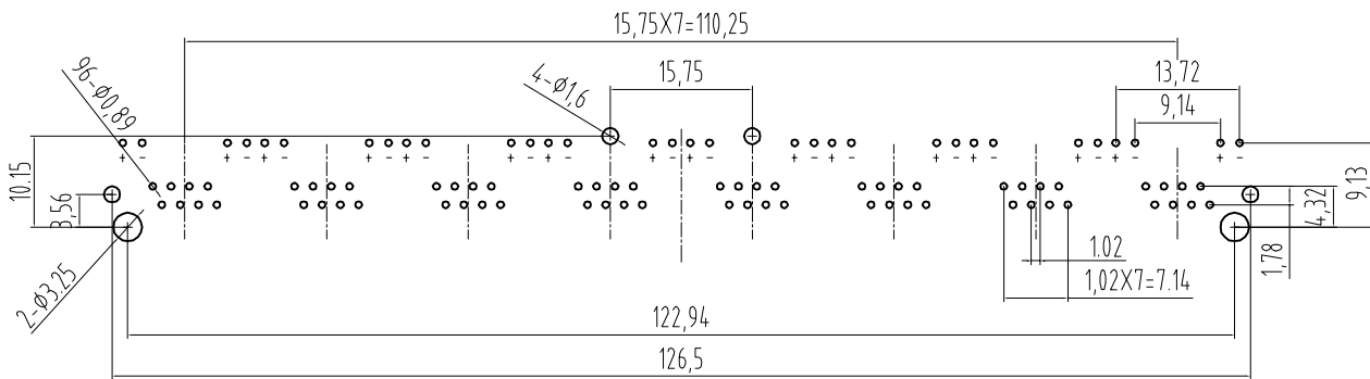
PC Board Layout Component Side Shown
