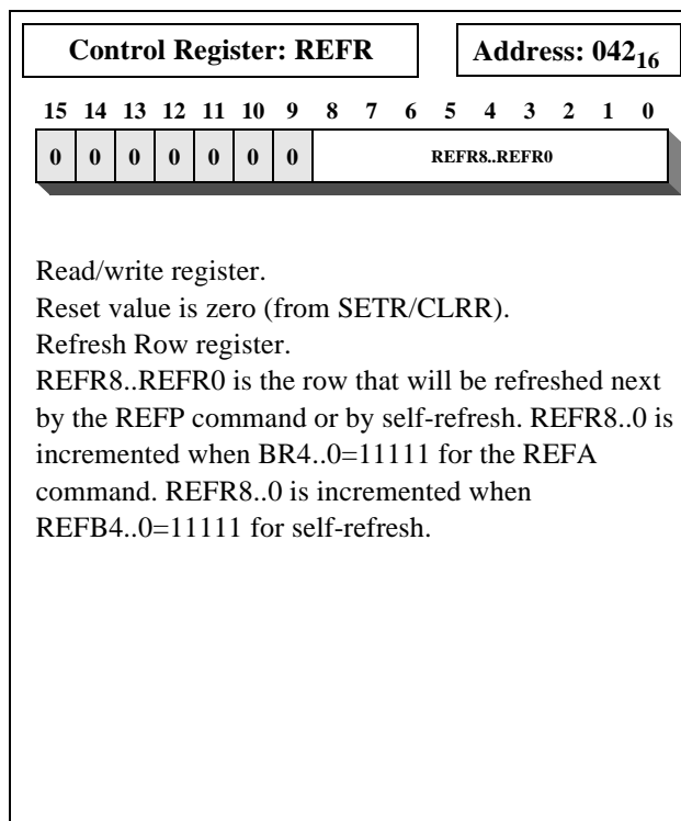
Figure 34: REFR Register
