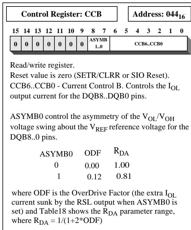
Figure 35: CCB Register
