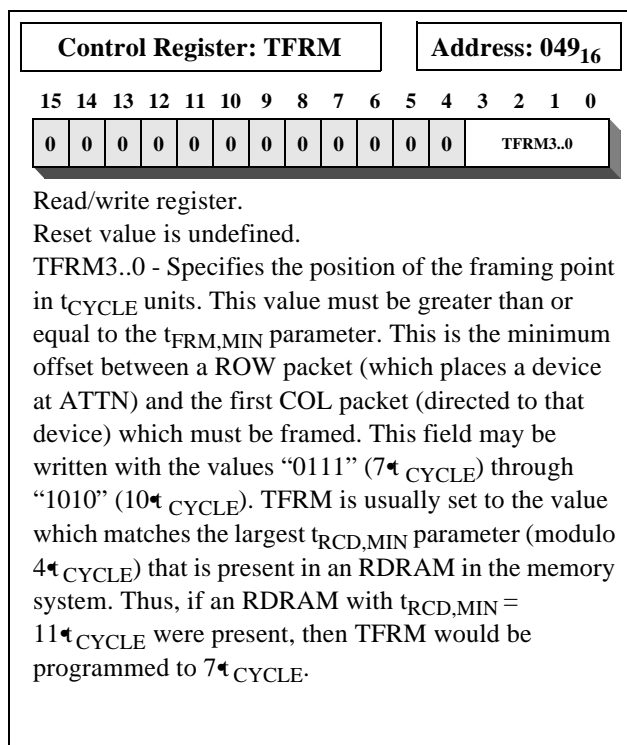
Figure 40: TFRM Register
