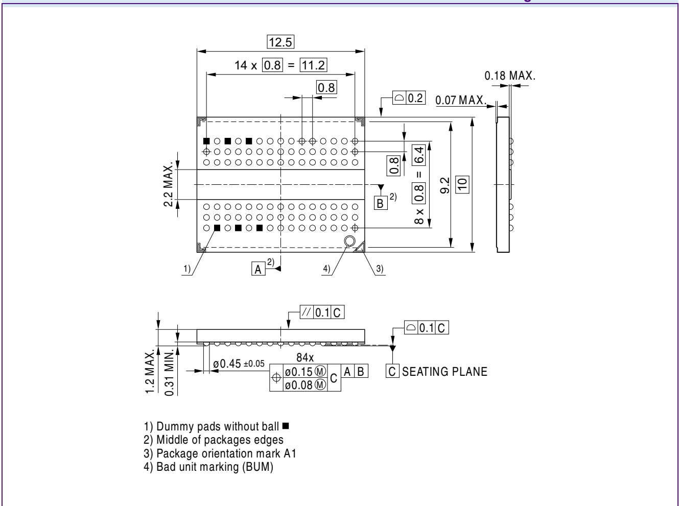
FIGURE 6 Package Outline P-TFBGA-84
