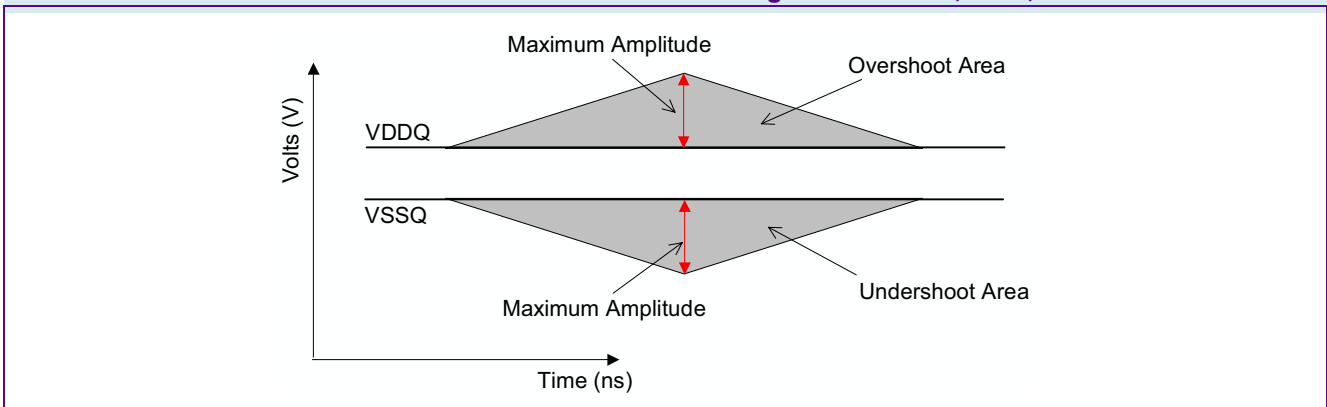
AC Overshoot / Undershoot Diagram for Clock, Data, Strobe and Mask Pins
