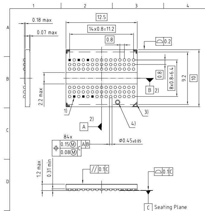
FIGURE 6 Package Outline P-TFBGA-84 (top view)
