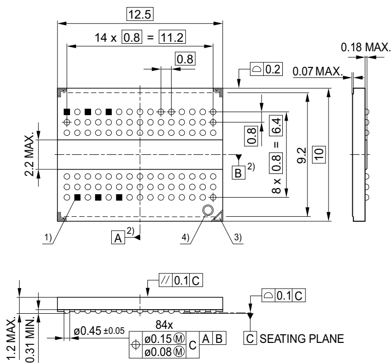
FIGURE 11 Package Outline P(G)-TFBGA-84-51
