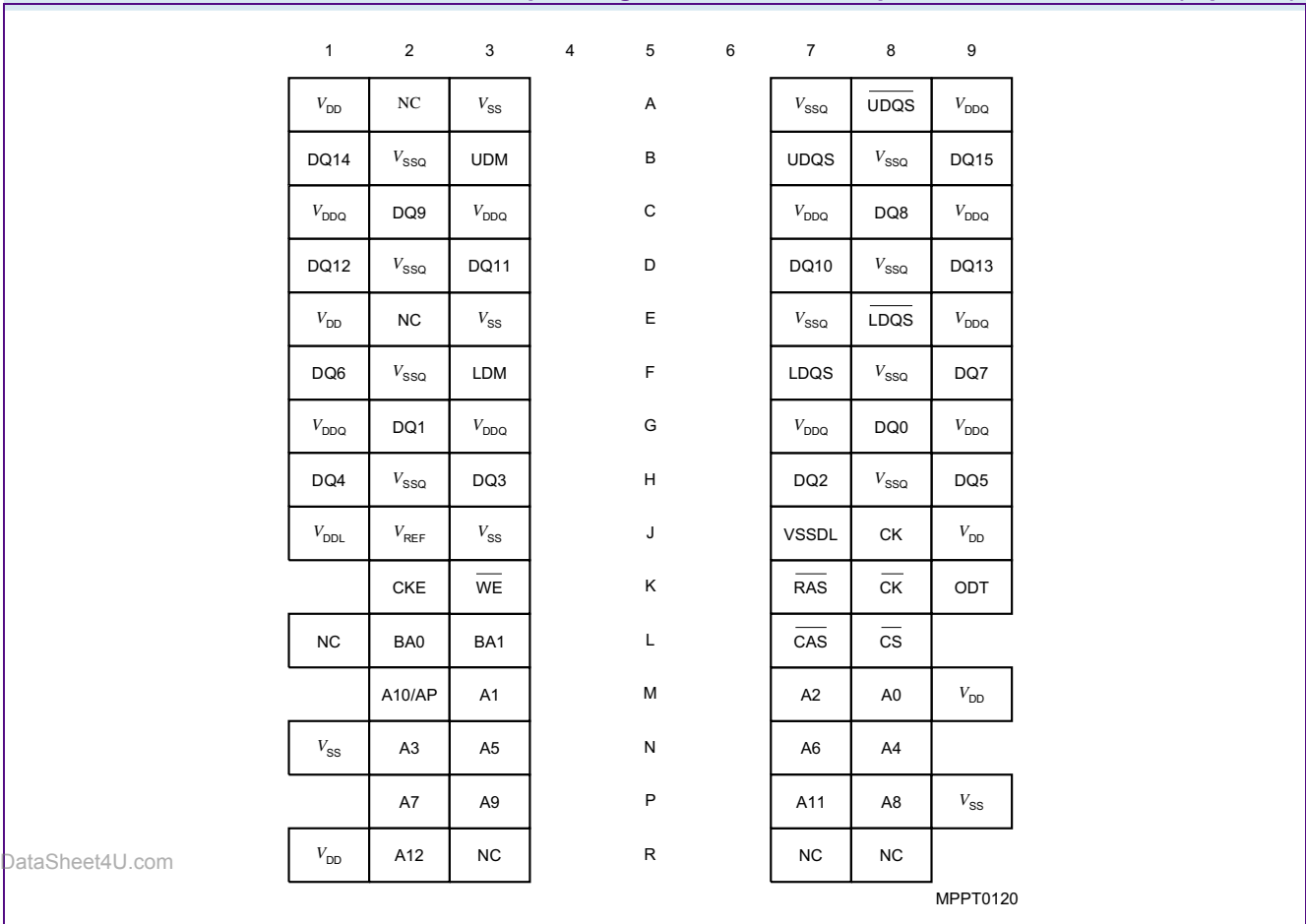
Chip Configuration for ×16 components, PG-TFBGA-84 (top view)
