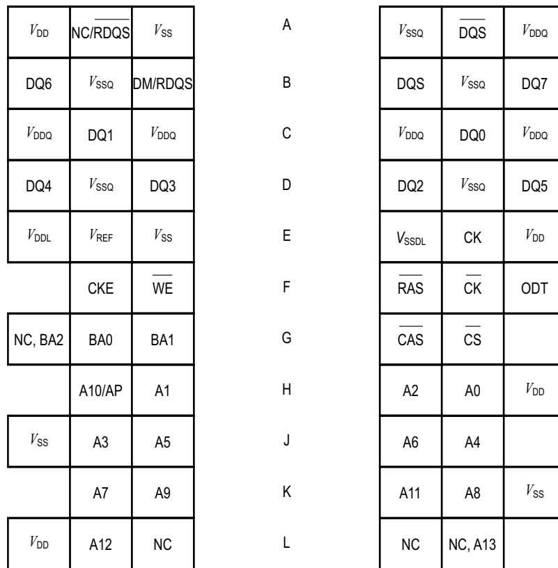
FIGURE 2 Chip Configuration for ×8 components, PG-TFBGA-60 (top view)
