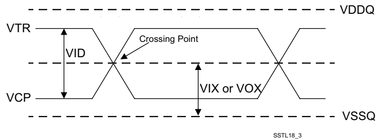
Differential DC and AC Input and Output Logic Levels Diagram
