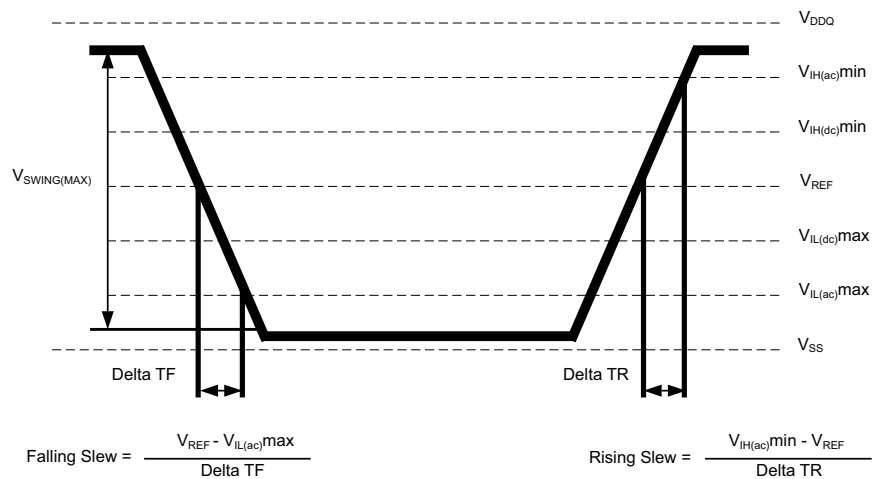
FIGURE 3 Single-ended AC Input Test Conditions Diagram
