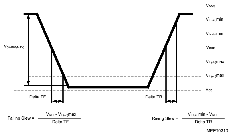
FIGURE 3 Single-ended AC Input Test Conditions Diagram
