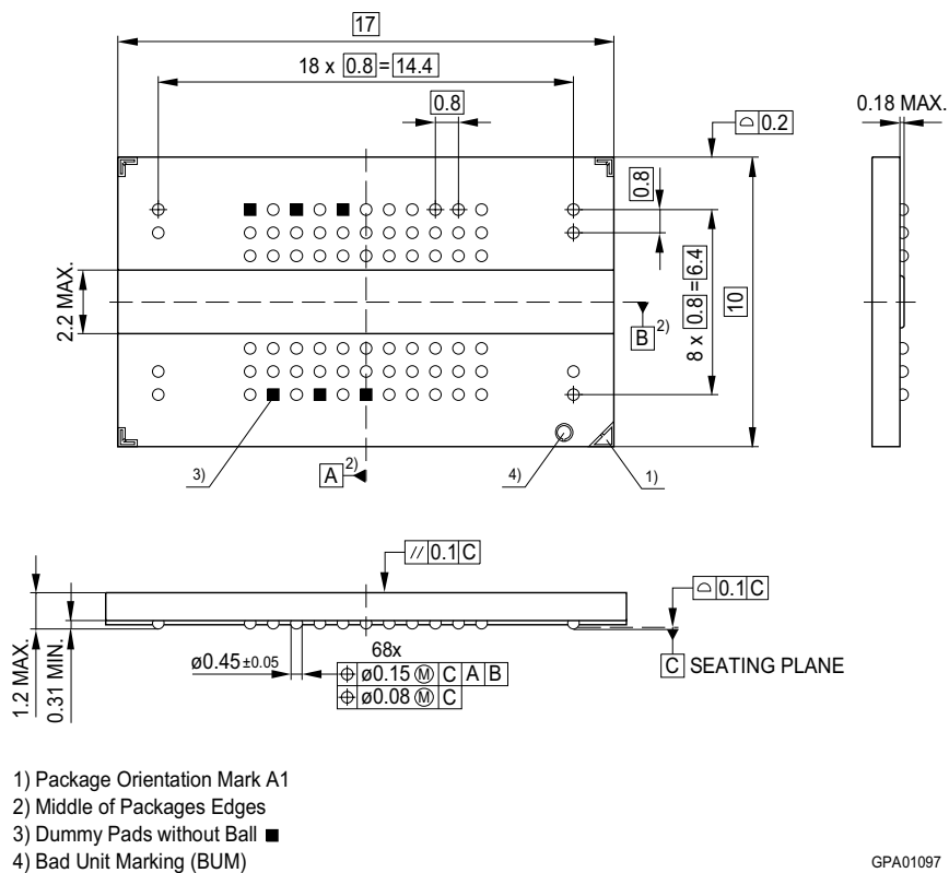
FIGURE 10 Package Outline PG-TFBGA-68
