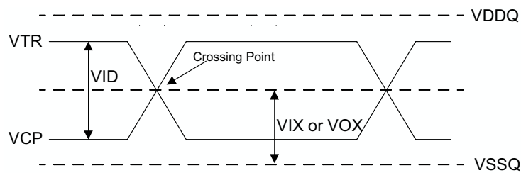
Differential DC and AC Input and Output Logic Levels Diagram
