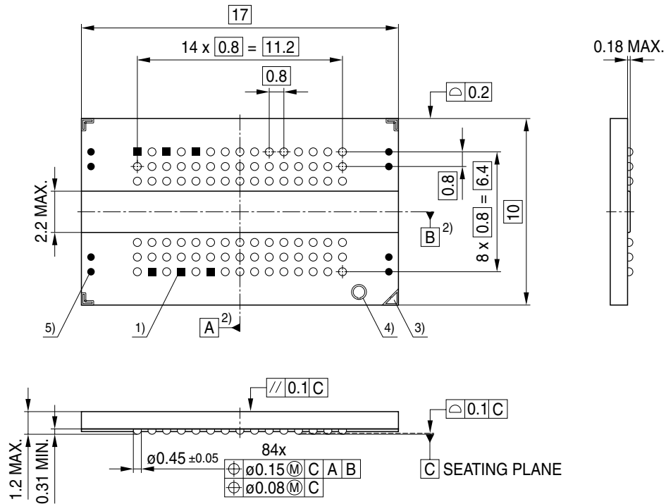
FIGURE 11 Package Outline PG-TFBGA-84
