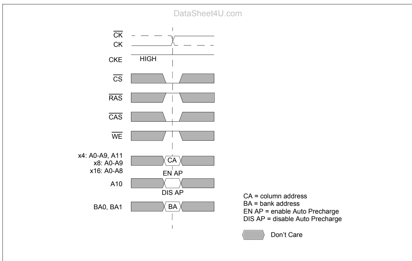
Figure 8 Read Command
