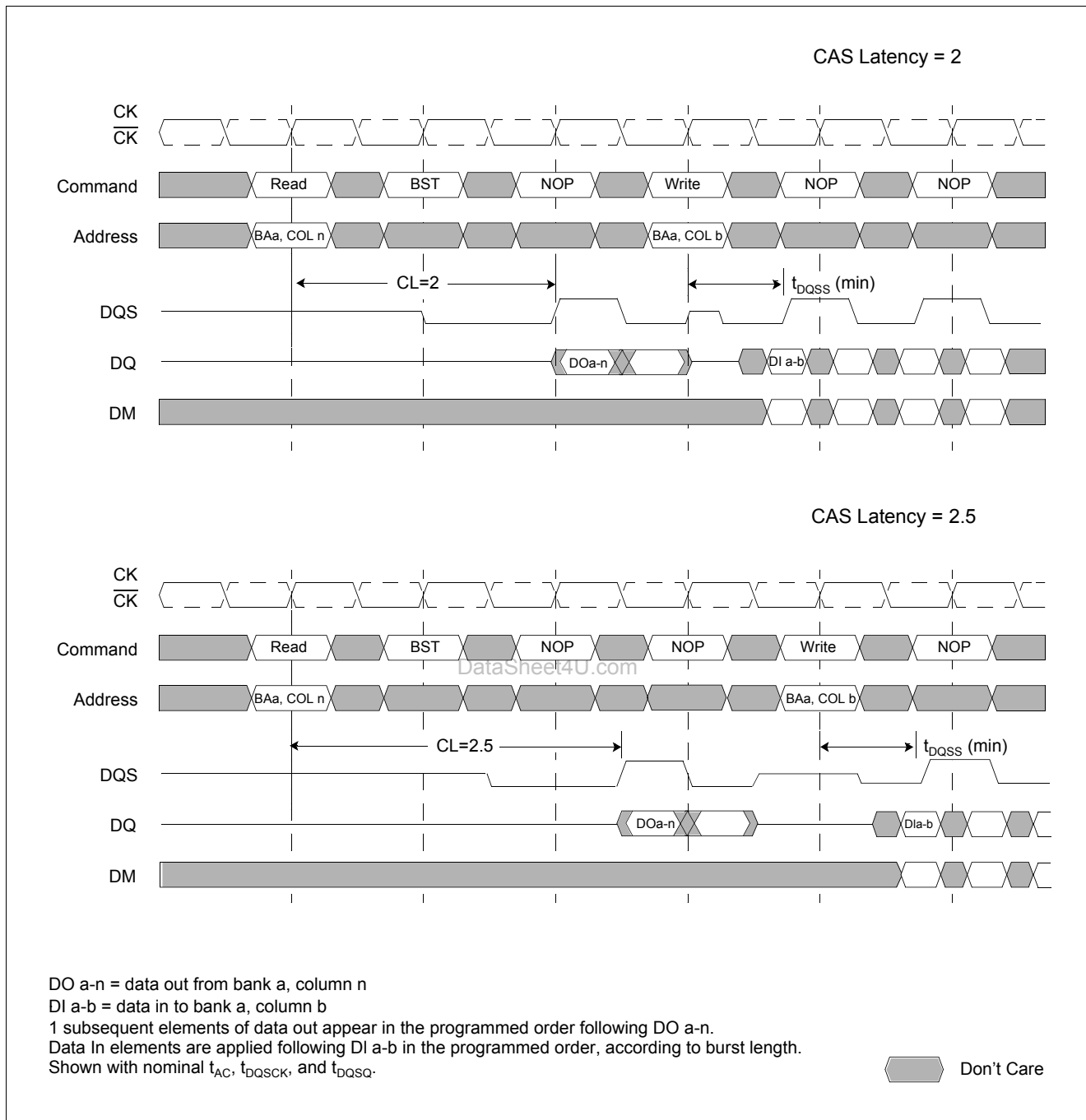
Figure 14 Read to Write: CAS Latencies (Burst Length = 4 or 8)
