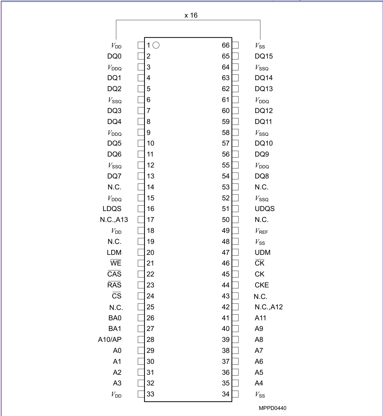
FIGURE 1 Chip Configuration PG-TSOP11-66
