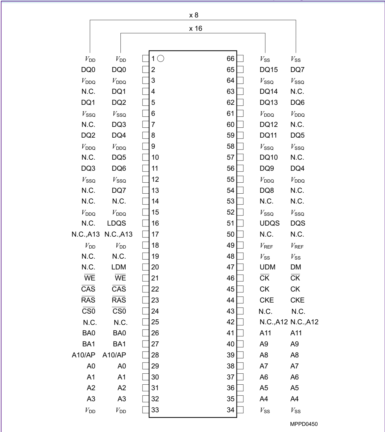
FIGURE 1 Chip Configuration PG-TSOPII-66
