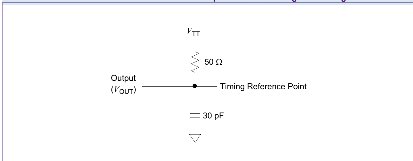
FIGURE 4 AC Output Load Circuit Diagram / Timing Reference Load
