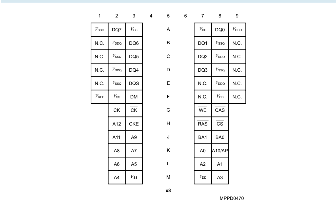
Pin Configuration for x8 Organization, PG-TFBGA-60, Top View
