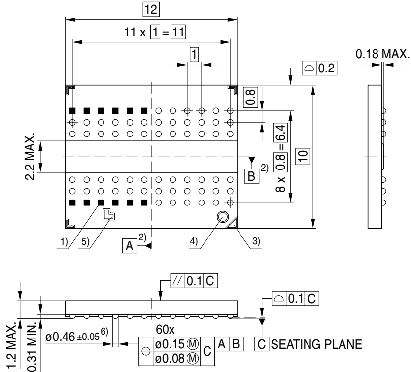
FIGURE 6 Package Outline P(G)-TFBGA-60
