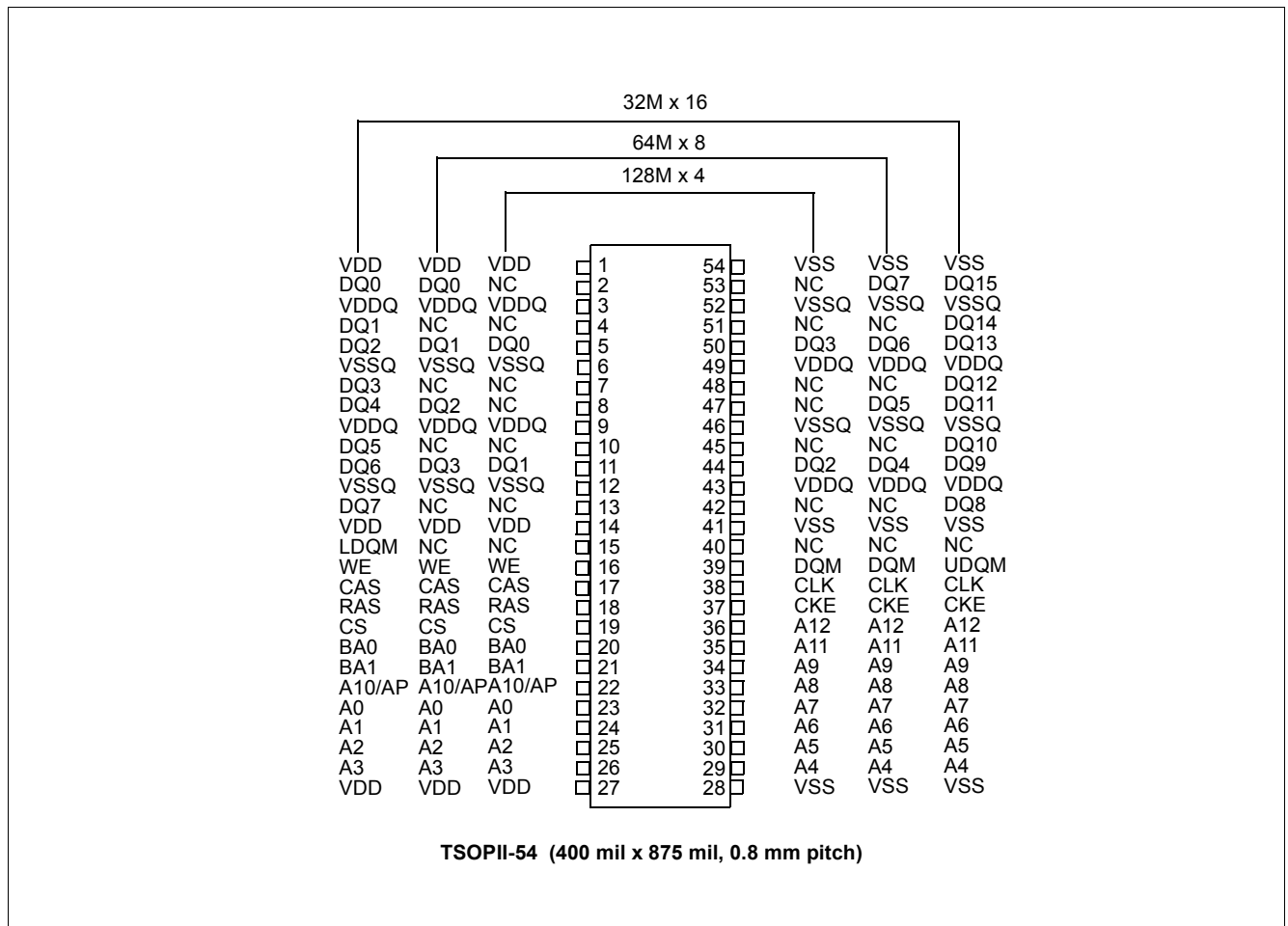
Figure 1 PinoutP-TSOPII-54
