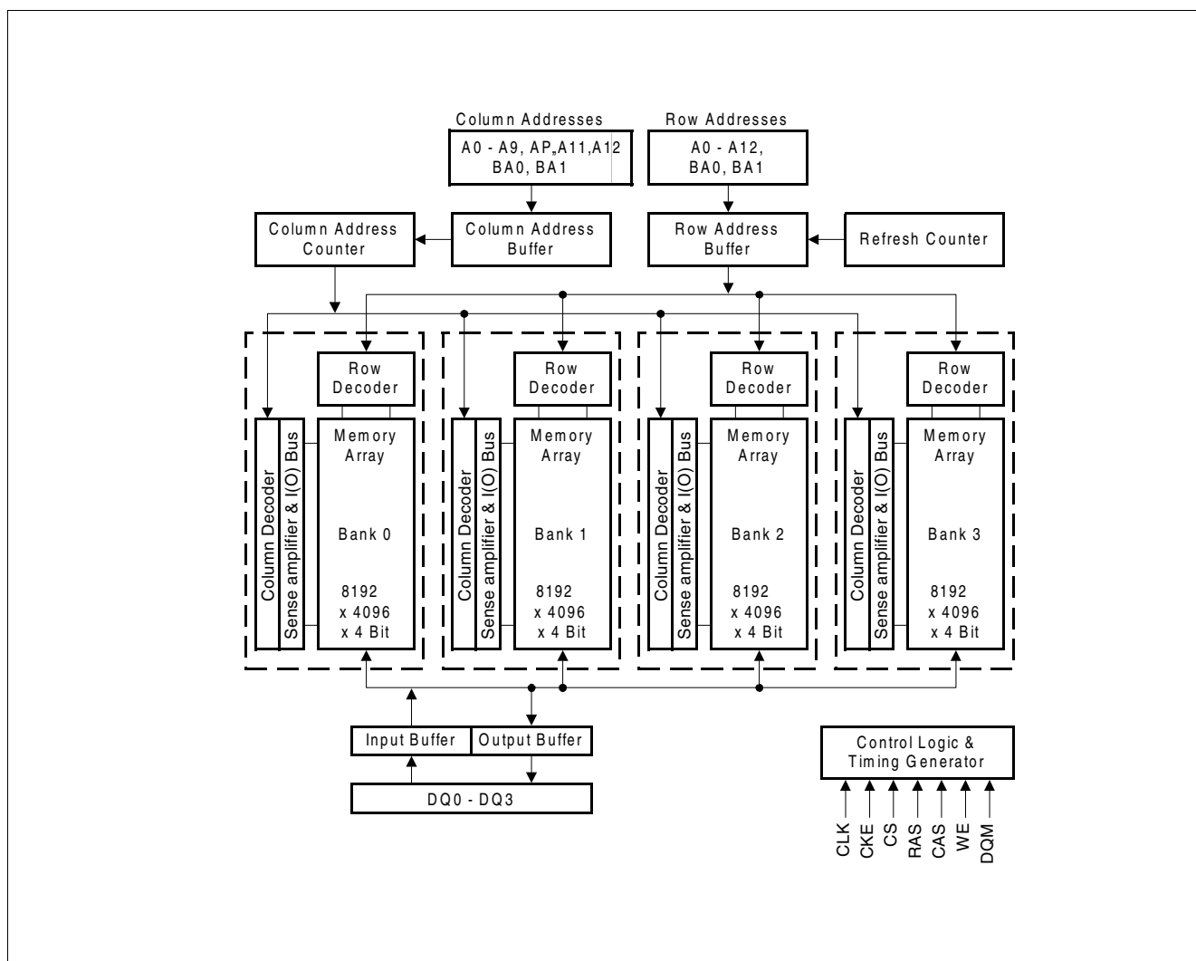
Figure 2 Block Diagram for 128M x 4 SDRAM (13 / 12 / 2 addressing)
