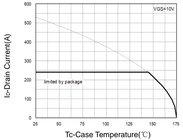
Figure 2: Drain Current
