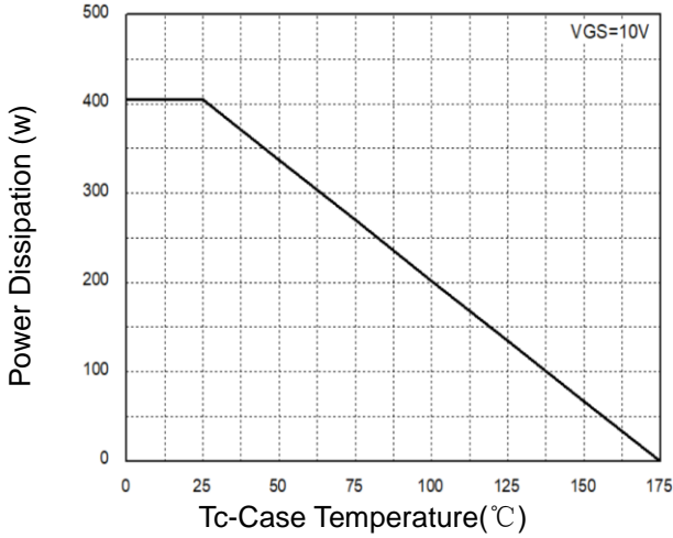
Figure 1: Power Dissipation
