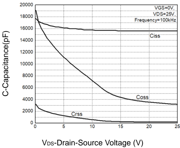
Figure 9: Capacitance Characteristics
