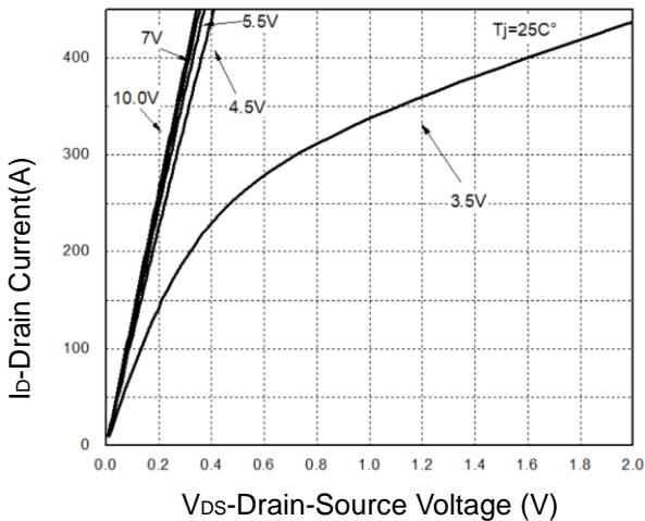
Figure 5: Output Characteristics
