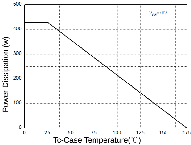
Figure 1: Power Dissipation
