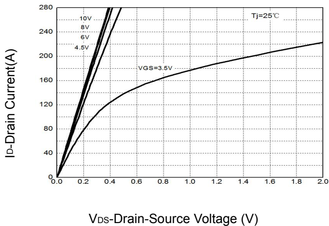
Figure 5: Output Characteristics
