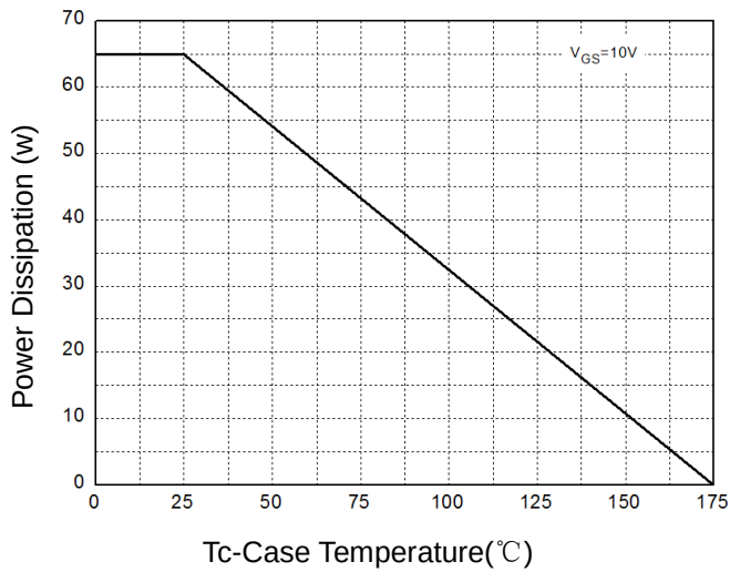
Figure 1: Power Dissipation
