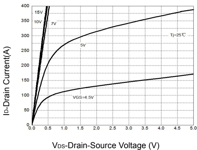
Figure 5: Output Characteristics
