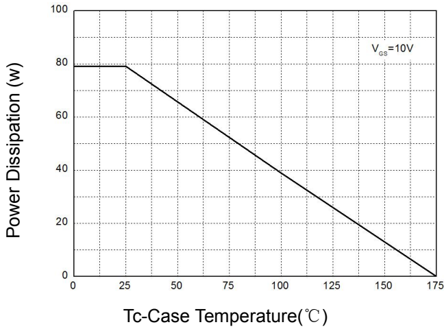
Figure 1: Power Dissipation
