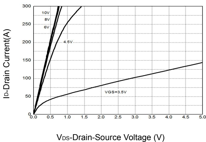
Figure 5: Output Characteristics
