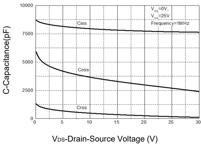
Figure 9: Capacitance Characteristics
