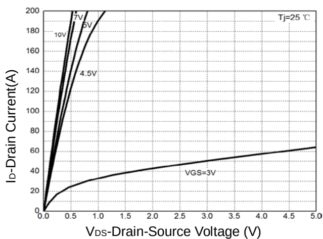
Figure 5: Output Characteristics
