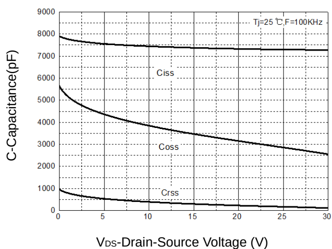
Figure 9: Capacitance Characteristics
