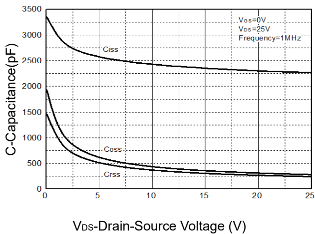
Figure 9: Capacitance Characteristics
