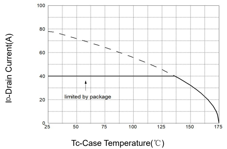
Figure 2: Drain Current
