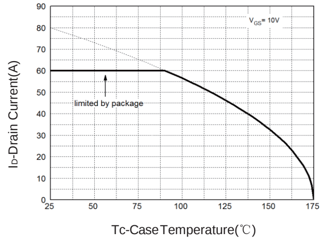
Figure 2: Drain Current
