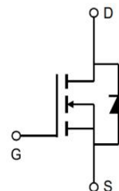
Single N-Channel MOSFET
