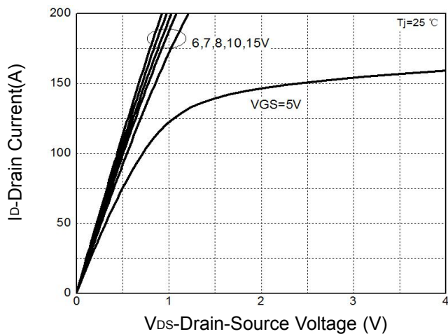
Figure 5: Output Characteristics
