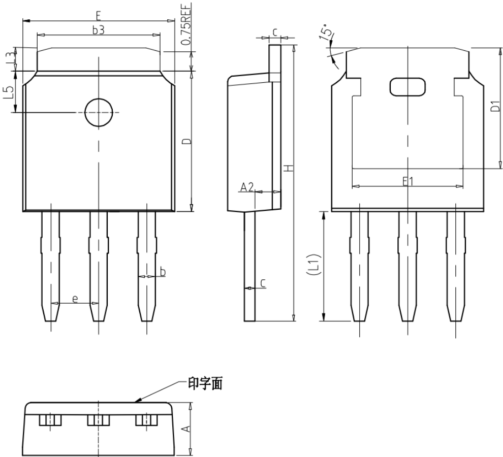
COMMON DIMENSIONS
