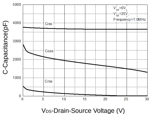
Figure 9: Capacitance Characteristics
