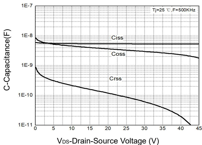
Figure 9: Capacitance Characteristics
