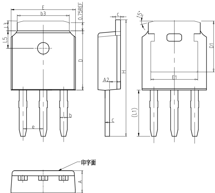
COMMON DIMENSIONS
