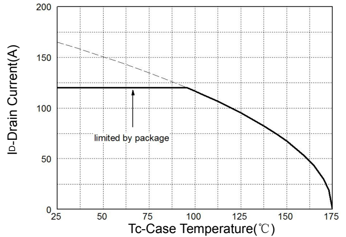
Figure 2: Drain Current
