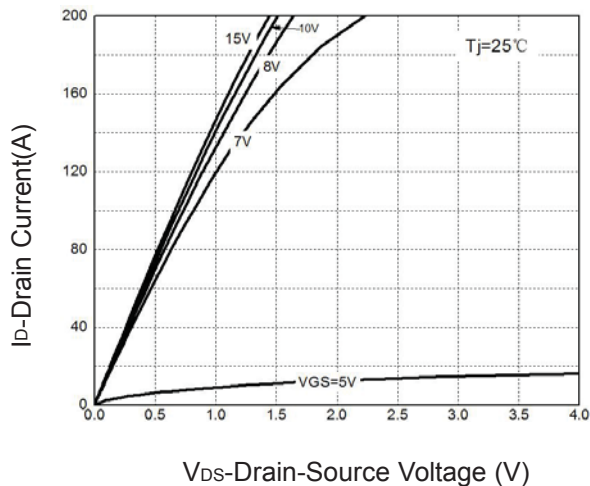
Figure 5: Output Characteristics
