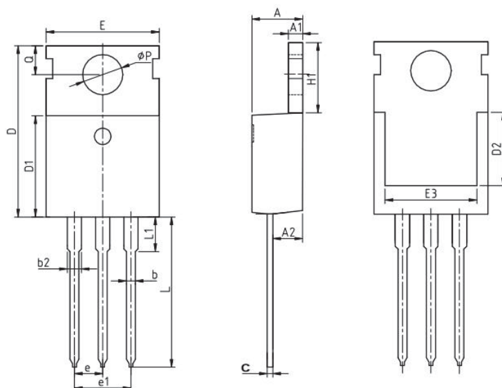
COMMON DIMENSIONS
