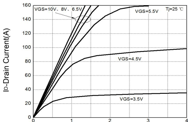
Figure 5: Output Characteristics
