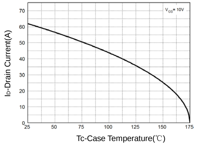
Figure 2: Drain Current
