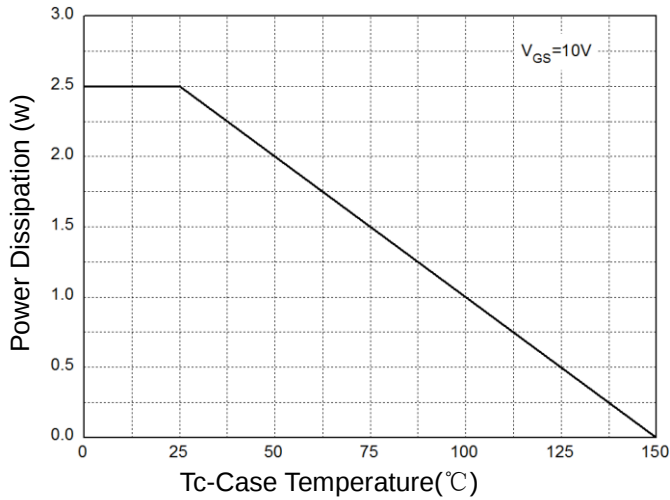
Figure 1: Power Dissipation
