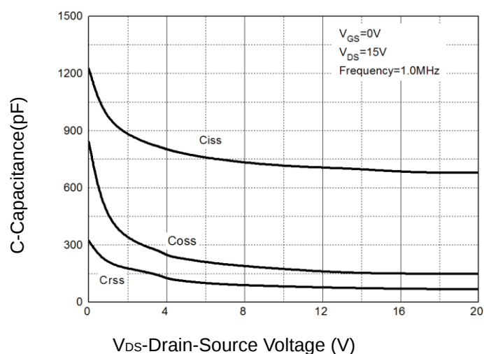
Figure 9: Capacitance Characteristics
