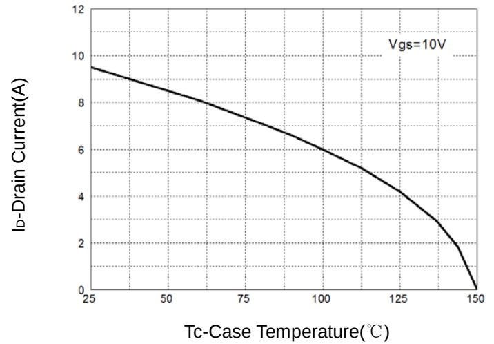
Figure 2: Drain Current
