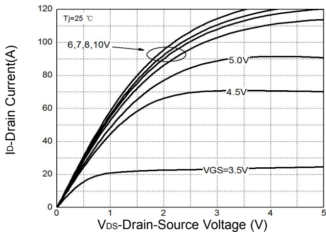
Figure 5: Output Characteristics
