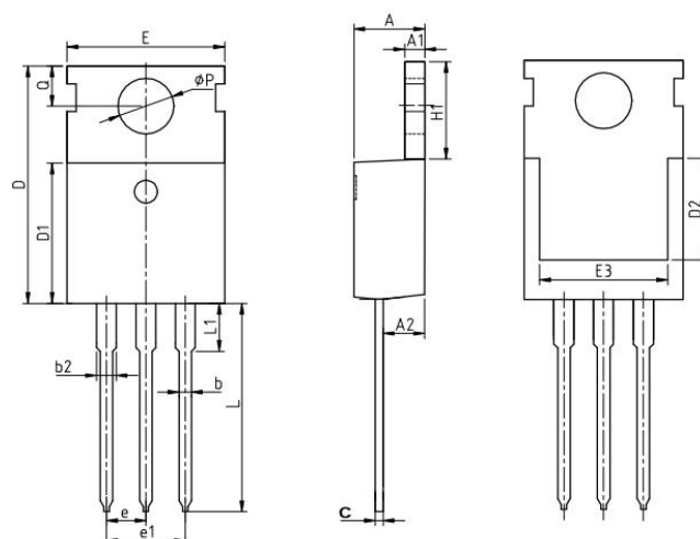
COMMON DIMENSIONS
