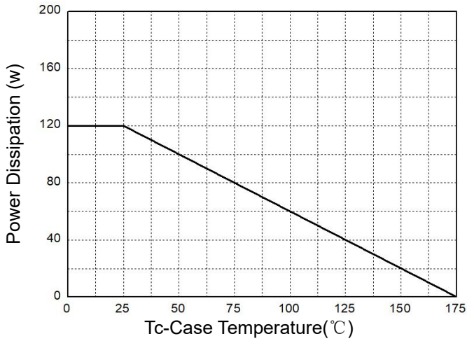
Figure 1: Power Dissipation
