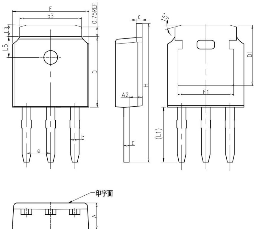
COMMON DIMENSIONS
