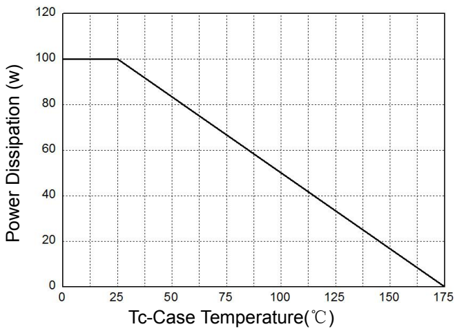
Figure 1: Power Dissipation
