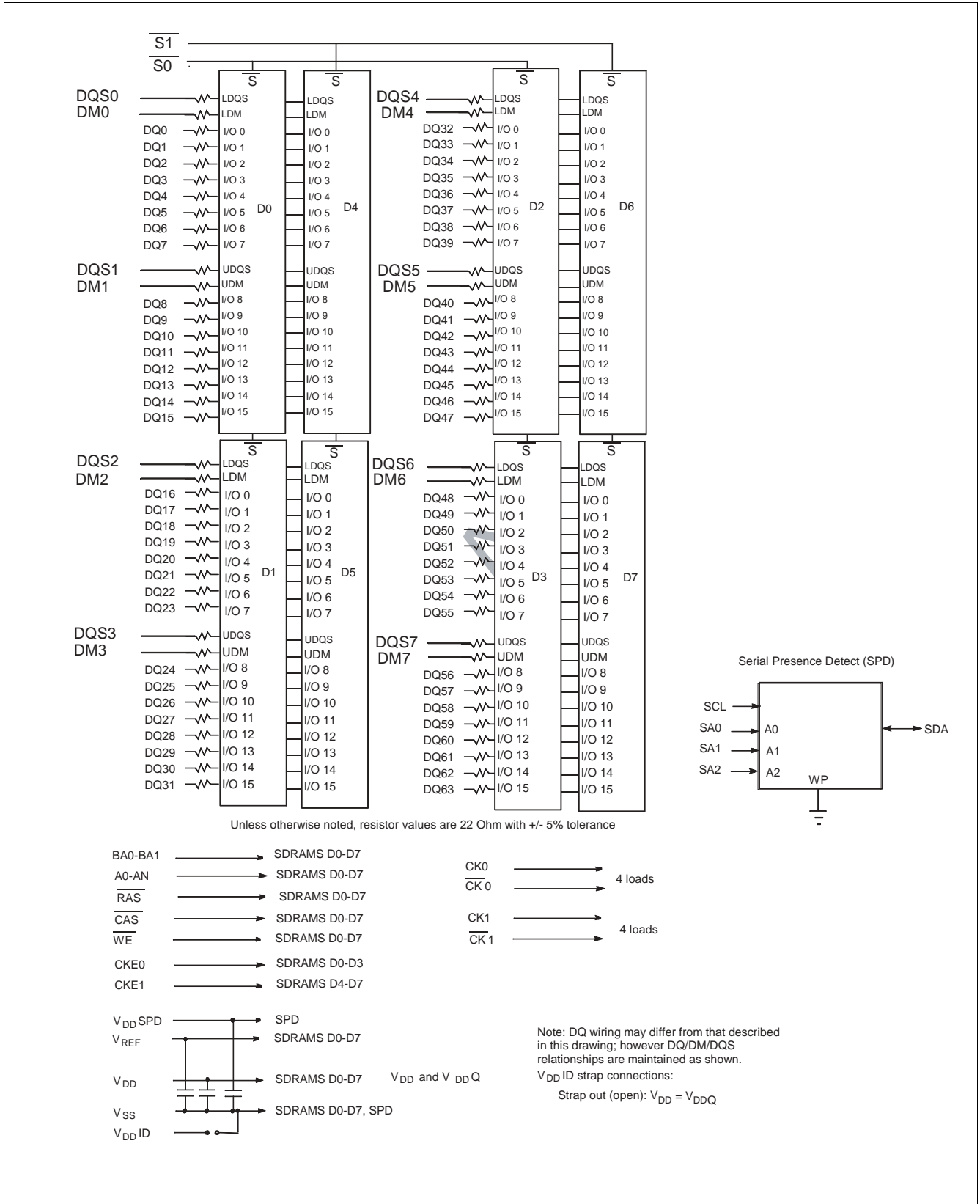
Figure 3 Block Diagram - Two Ranks 32M x 64 DDR SDRAM SO-DIMM HYS64D32020HDL-6-C
